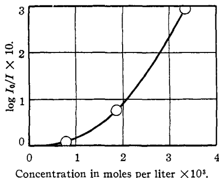
Fig. 4.—Peroxide calibration.
